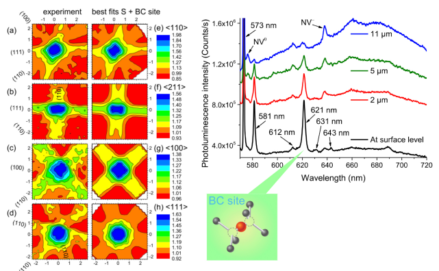
Figure 1: (a)–(d): Experimental \beta^- EC patterns from ^{121}\text{Sn} implanted diamond following 920°C annealing. (e)–(h): corresponding best fits of theoretical patterns considering 79% on ideal substitutional and 32% on ideal BC sites. Right: confocal PL spectra following the decay of ^{121}\text{Sn} to ^{121}\text{Sb} , i.e., \text{SnV}^- related lines, with the major component at 621 nm, result from long-lived ^{121\text{m}}\text{Sn} . The spectra were recorded at room temperature under 532 nm laser excitation with the focus at various depths. Bottom center: The atomic structure of \text{SnV}^- in the split-vacancy configuration.
