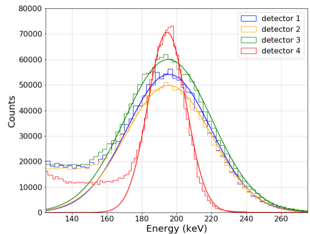
Figure 3: Calibrated spectra of 129m Xe decay registered with the four detectors. Single Gaussian fitting was applied and the area under the fits was used to determine the gamma asymmetry value.
